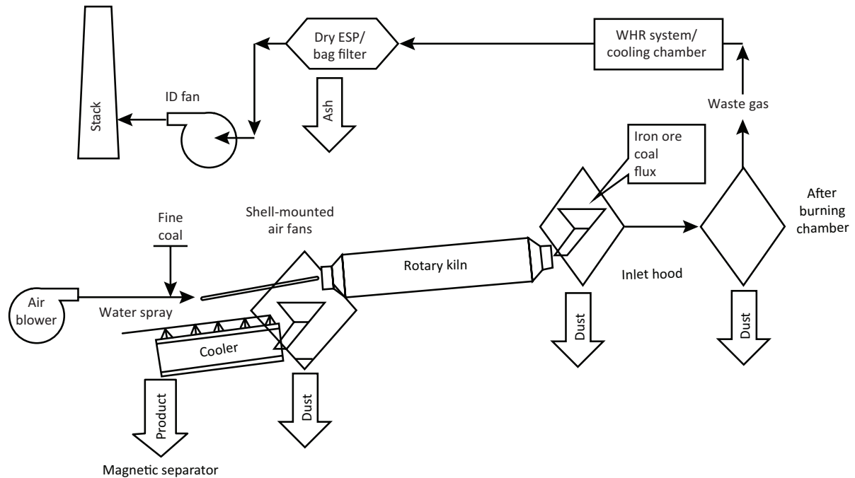
Figure 36: Schematic layout of DRI manufacturing process
