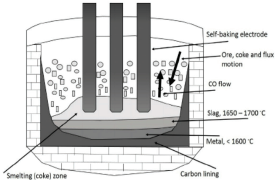
Figure 62 : View of submerged arc furnace
