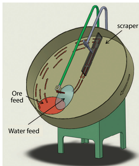
Figure 23: Pictorial view of a balling disc
