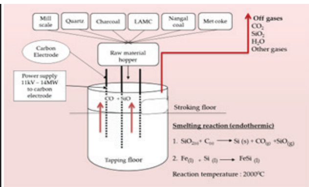
Figure 68 : Production process of ferro silicon
